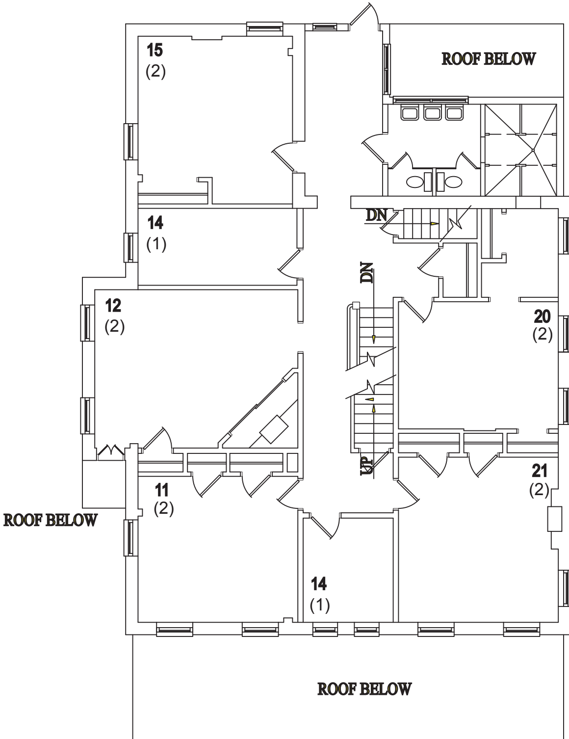
CARLISLE HOUSE SECOND FLOOR PLAN
