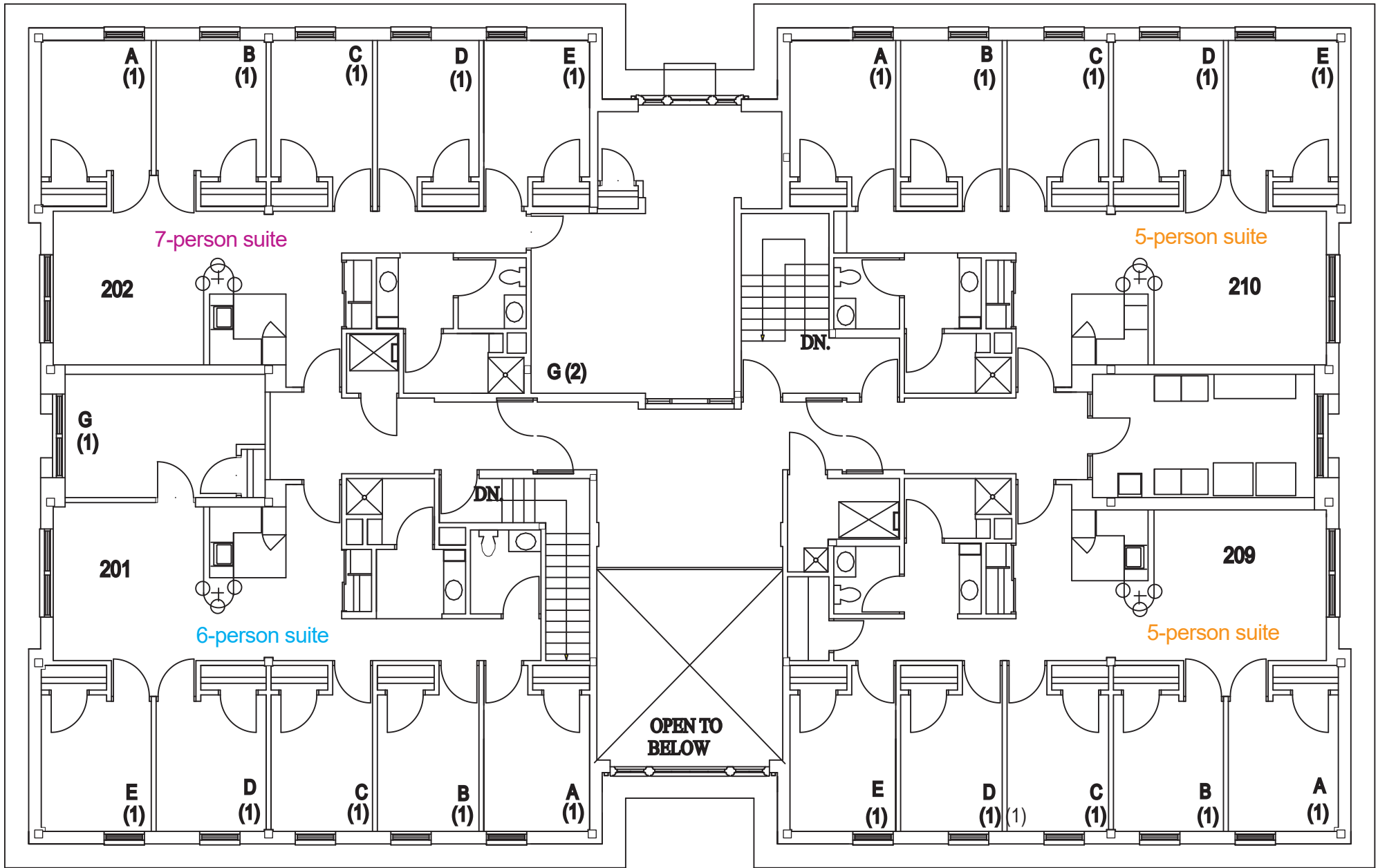
QUARRY SUITE WEST SECOND FLOOR PLAN
