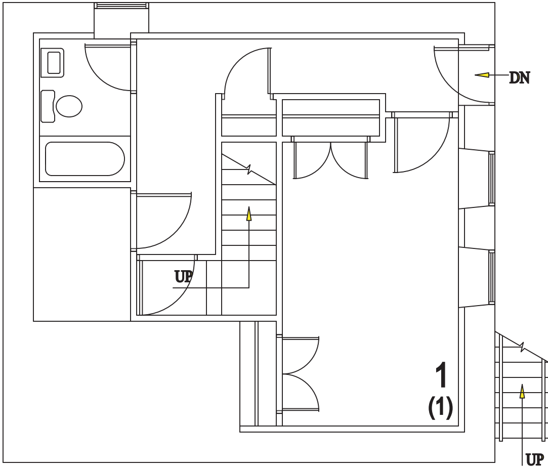
LAU HOUSE Basement Floor Plan
