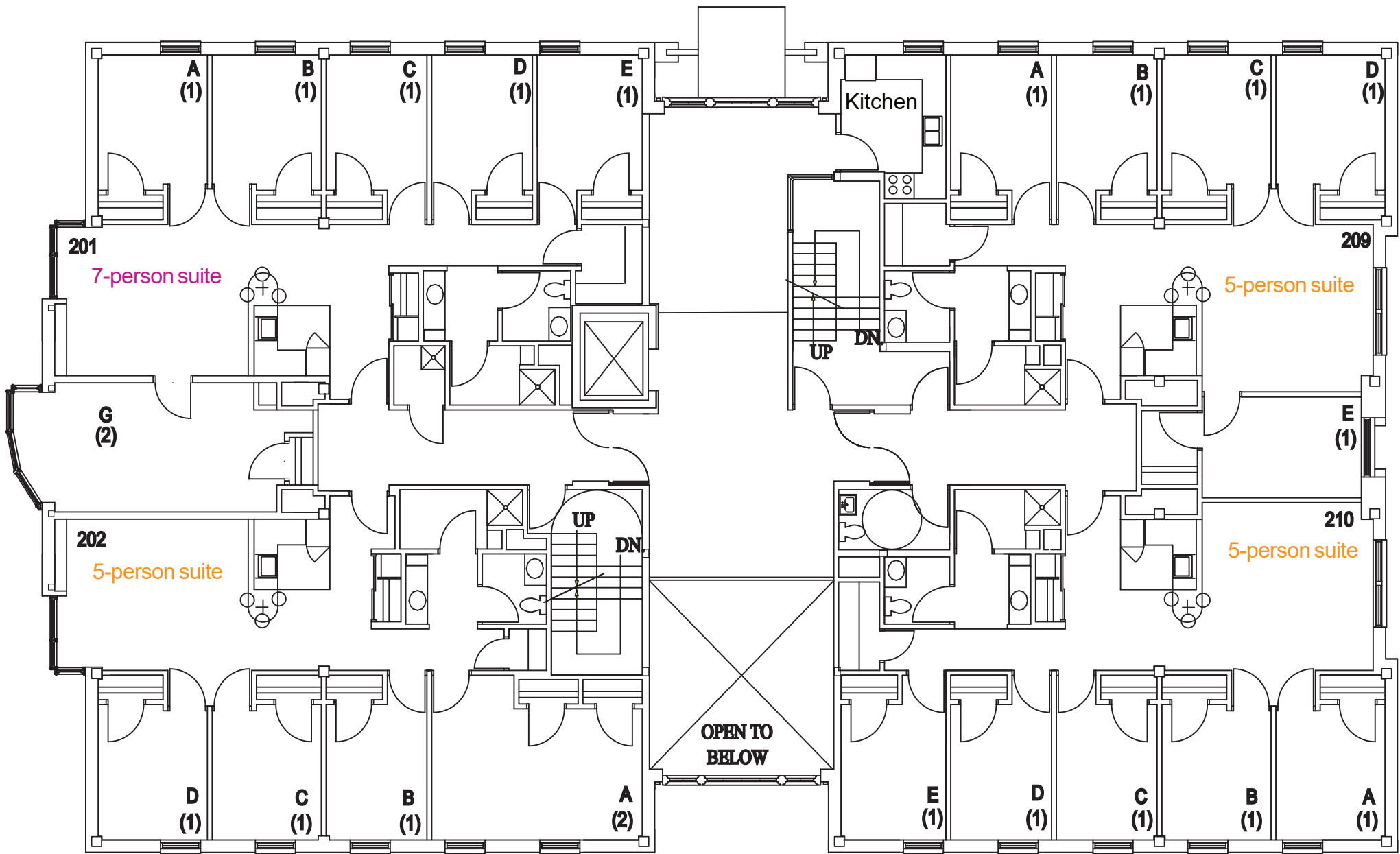
HAALAND HALL SECOND FLOOR PLAN - SOUTH BUILDING
